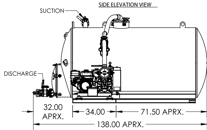
TVP-1000-S, SIDE MOUNTED, 230 CFM DIMENSIONAL DRAWING
