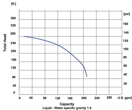
Performance of 2" High Pressure Pumps
