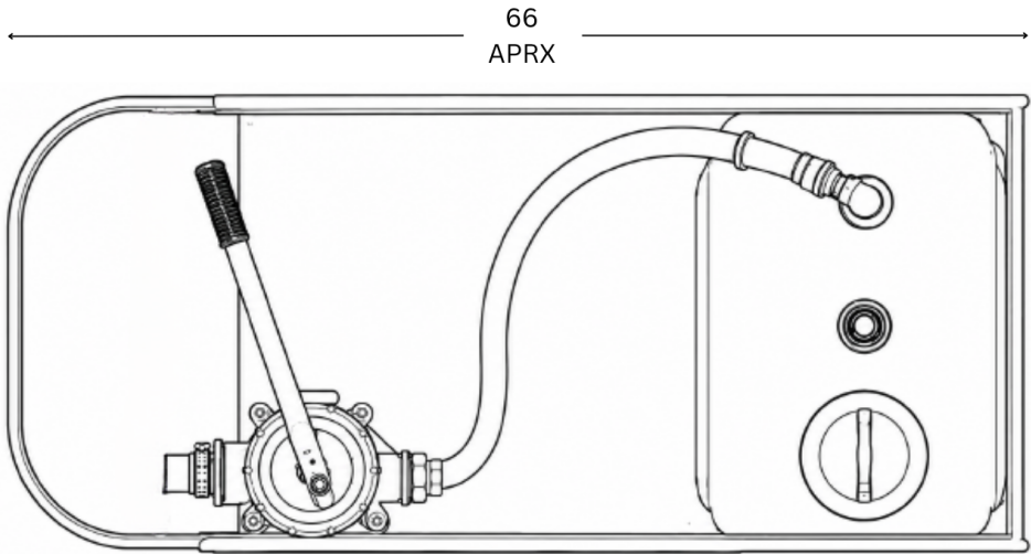
TOP ELEVATION VIEW
